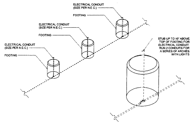
4 TRENCH - CONDUIT STUB-UP
