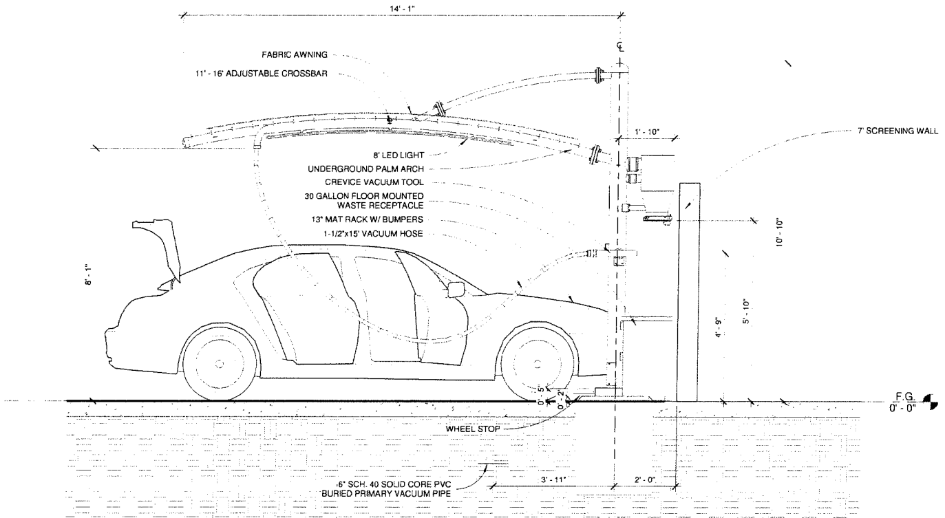
3 TYPICAL PARKING ELEVATION
