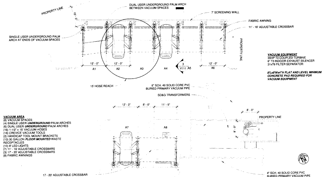
SITE PLAN
