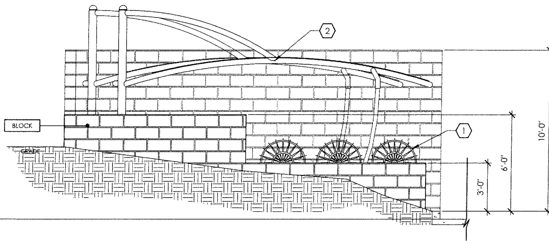
A NORTH PLANTER BLOCK WALL ELEVATION
