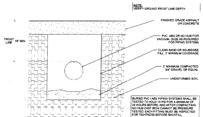
6 TRENCH - SINGLE LINE
