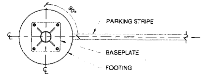
2 BASEPLATE ORIENTATION 1/2" = 1'-0"
