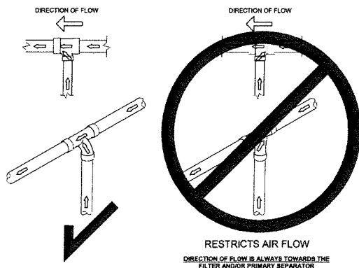
3 PIPE - PIPE FLOW
