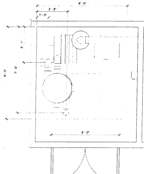
2 EQUIPMENT DIMENSIONS
